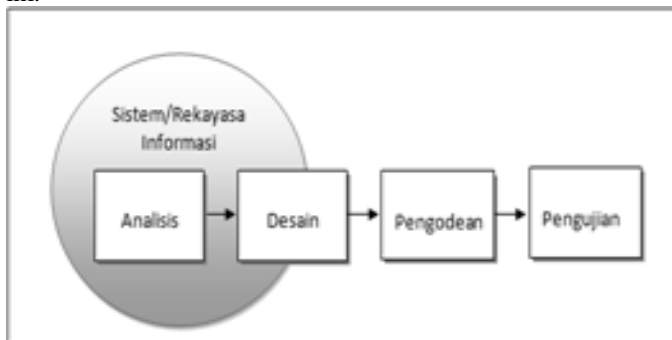
Gambar 1. Metode Waterfall
