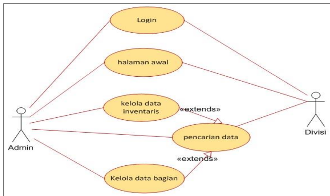
Gambar 2. UsecaseDiagram Sistem
