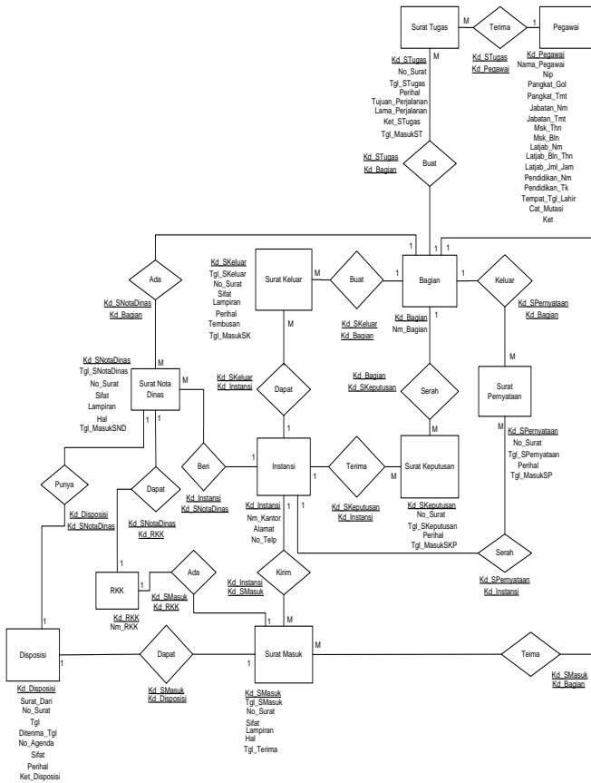
Gambar 7 Entity Relationship Diagram (ERD)
