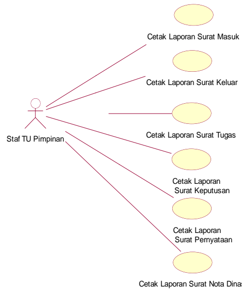
Gambar 6 Use case diagram laporan
