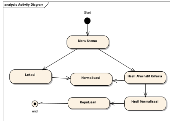
Gambar 3. Activity Diagram
