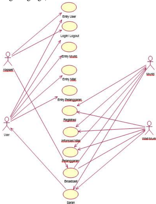
Gambar 4. Use Case Master
